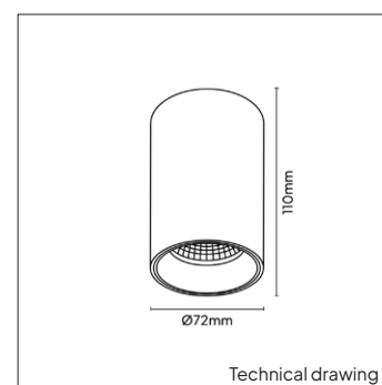
Technical drawing
