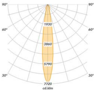
15° (2625-00010)
